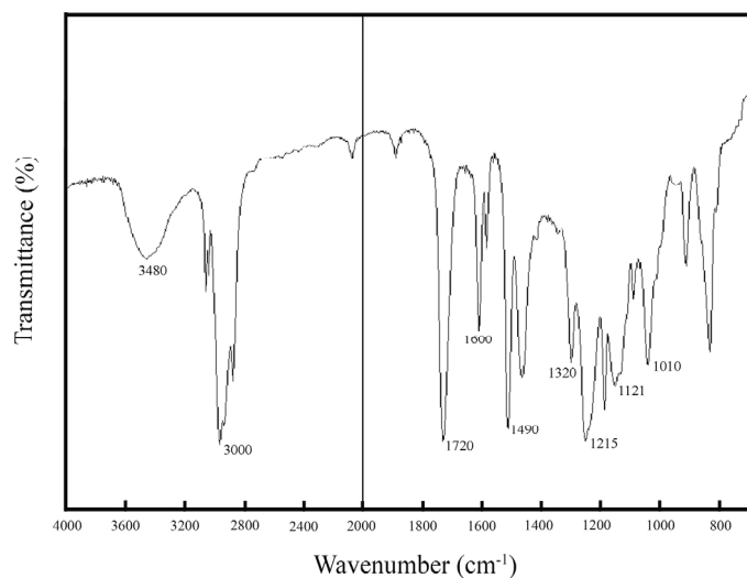
Fig. 2. FTIR spectrum of poly ortho aminophenol structure.
