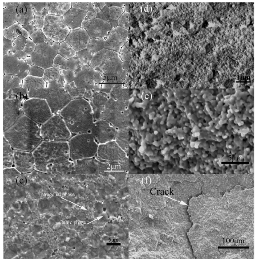
Fig. 4. SEM micrograph of pure 8YSZ (a), 7.6YSZ net (b), 6.9YSZ net (c), porous body after binder removal at 600 °C (d), impregnated body after annealing at 800°C (e) and fracture surface of some impregnated bodies (f)
