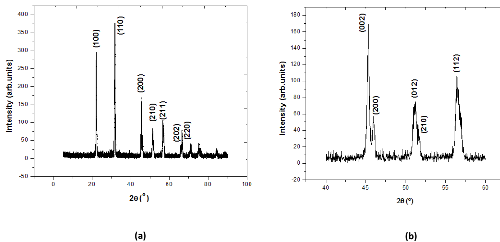
Fig. 11. Diffraction pattern of microwave sintered KNN ceramic, (a) Full scan of 2\theta and (b) Selected part showing XRD patterns between 40° to 60° 2\theta .
