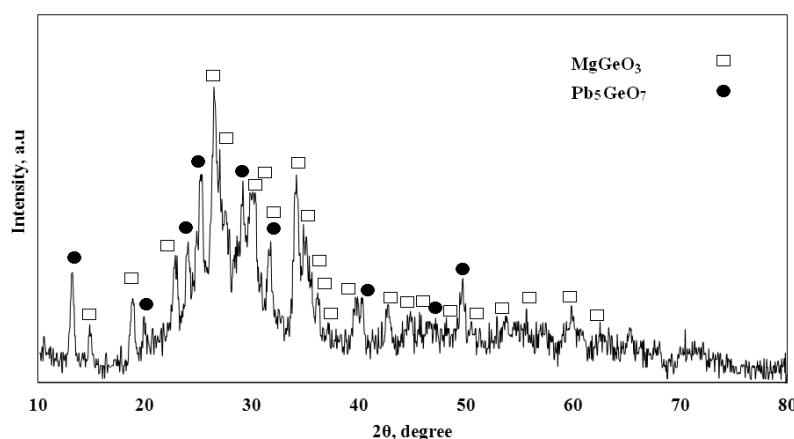
Fig. 4. The XRD pattern of as-quenched 65\text{GeO}_2\cdot 15\text{PbO}\cdot 10\text{MgO}\cdot 10\text{MgF}_2 sample after annealing at 800^\circ\text{C} for 60 minutes.
