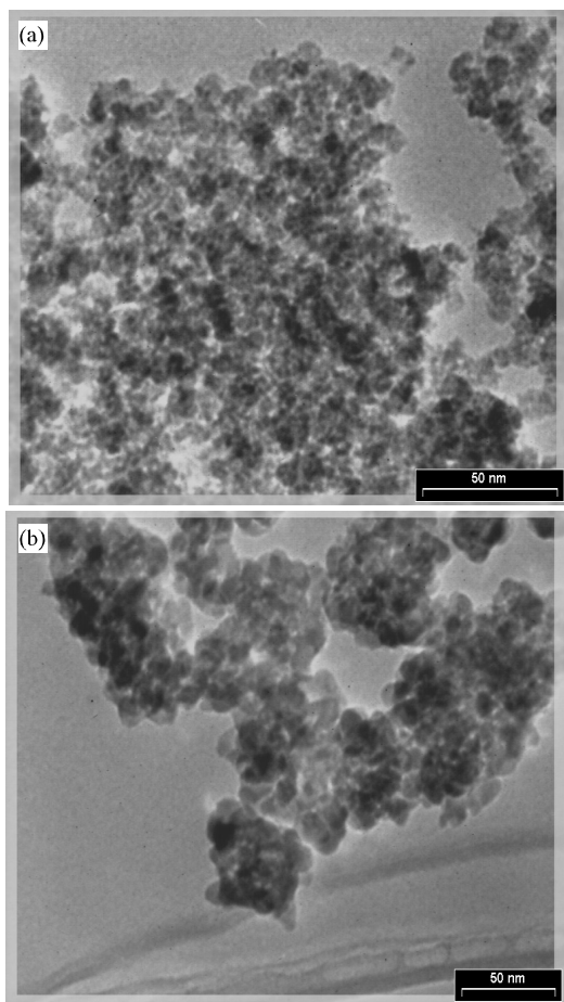
Fig. 2. TEM micrograph of \text{ZnFe}_2\text{O}_4 nanoparticles (a) synthesized at 80 °C and (b) synthesized at 80 °C and post calcined at 500 °C.
