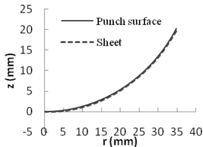
Fig. 10. Final geometry of the sheet on the punch.
