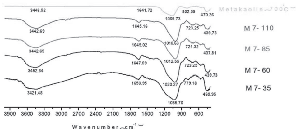
Fig. 5. FTIR spectra of the metakaolin calcined at 700 ^{\circ}\text{C} and geopolymer cements after 28 days curing with different molar ratio of \text{Na}_2\text{O}/\text{SiO}_2 .
