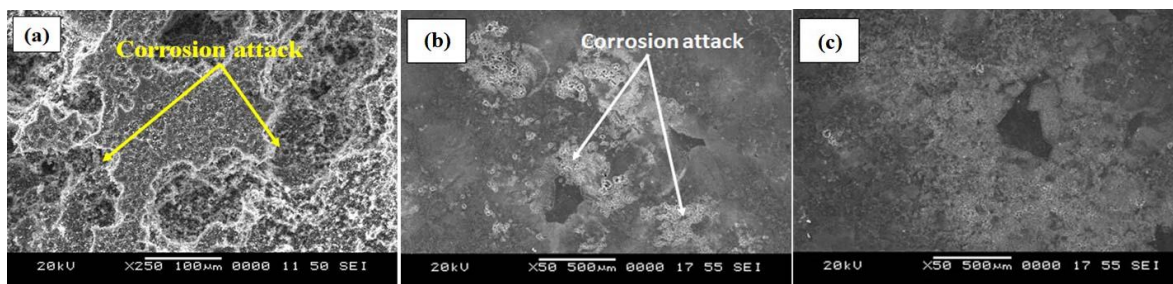
Fig. 8. Corrosion morphologies for AZ91 alloys a) as-supplied b) ECAP-2P c) ECAP-4P
