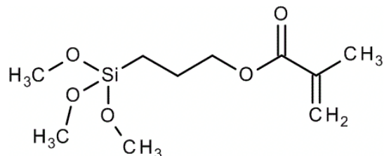
Fig. 1. Chemical structure of Silane A 174 [21]
