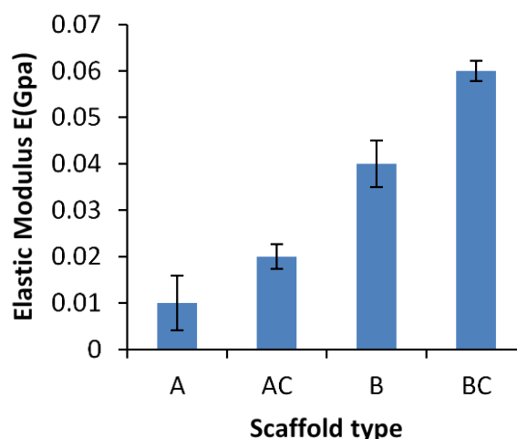
Fig. 4. Elastic modulus for uncoated and coated scaffolds
