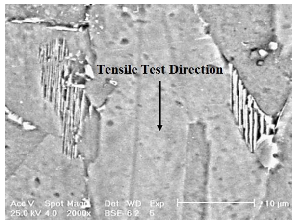
Fig. 8. The SEM image of the \eta phase elongation after the HTT in sample A286.
