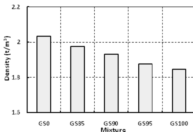
Fig. 5. Paste density at saturated surface dry condition at age of 28 days
