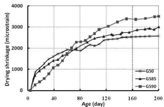
Fig. 12. Drying shrinkage of GS0, GS85 and GS90 paste prisms
