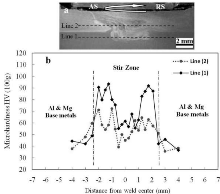
Fig. 11. Hardness distribution one mm above and below the lapping line in the sample welded at rotation speed of 1600 rpm and line speed of 40 mm/min.
